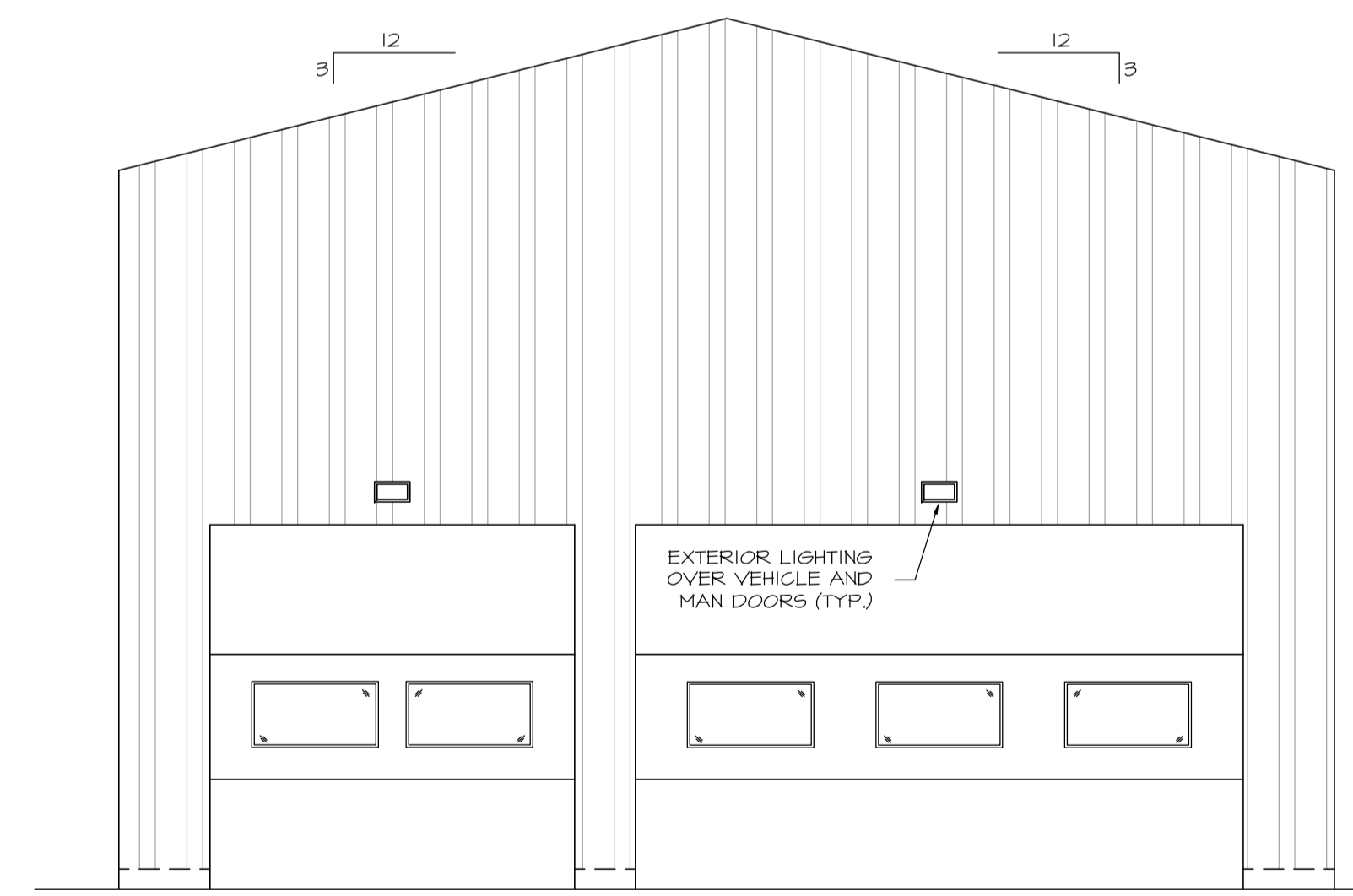
WEST ELEVATION SCALE: 3/16" = 1'-0"
