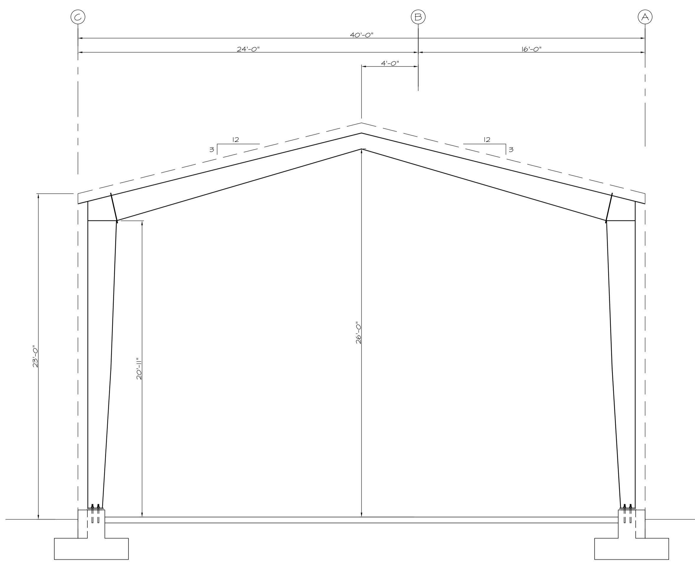
TYPICAL SECTION SCALE: 1/4" = 1'-0"
