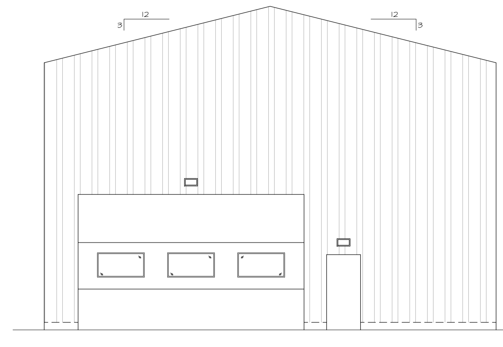
EAST ELEVATION SCALE: 3/16" = 1'-0"
